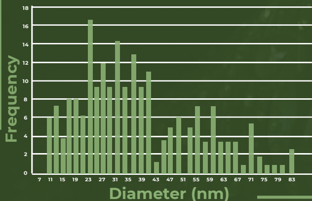
Histogram
