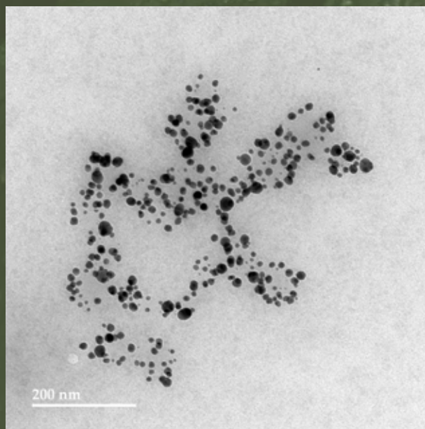
TEM Image of MOR-AG-00029
