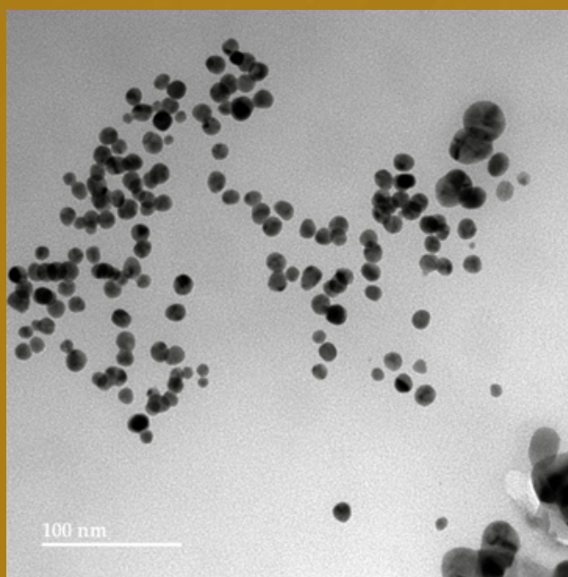
TEM Image of TMR-AG-00122
