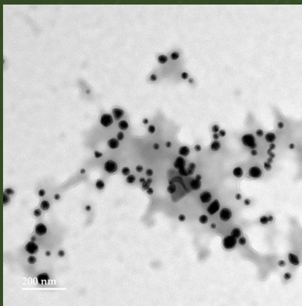
TEM Image of GRP-AU-00007
