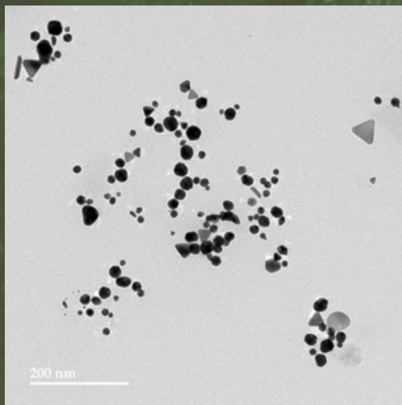
TEM Image of CFB-AU-00138
